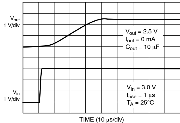
Figure 22. Startup Transient ( V_{out} = 2.5\text{ V} )
